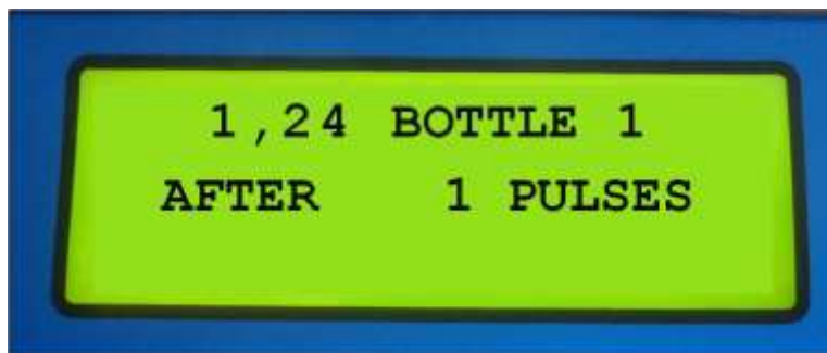
Figure 10. Autosampler default display screen for a resumed/restarted program. This shows that when triggered again from the datalogger, the sampler will begin with 1 of 24 pulses on bottle #1.
