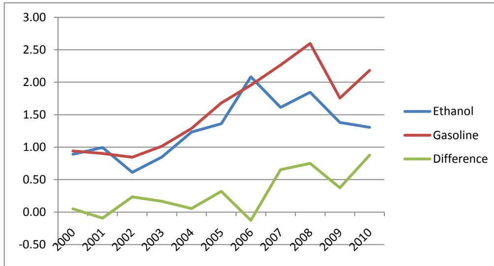
Figure 2. Minnesota's 10-Year Ethanol 23 vs. Gasoline 24 Price Trends, 2000-2010 25
